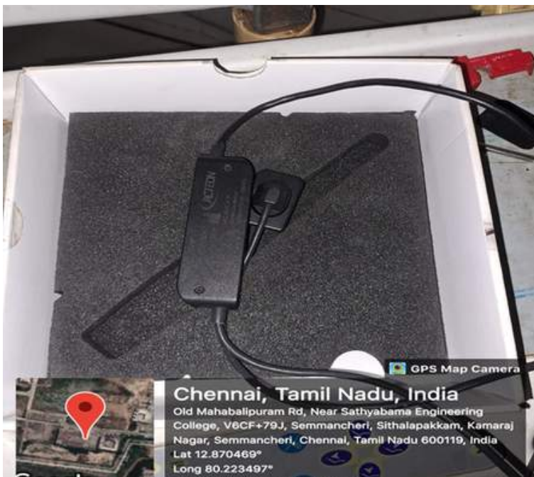
Radiovisuograph with CCD Sensor
